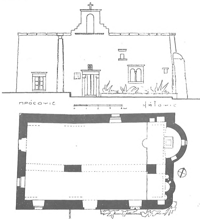
Εἰκ. 8. Ἡ κάτοψις καὶ ἡ πρόσοψις τοῦ ναοῦ τοῦ Χριστοῦ.
